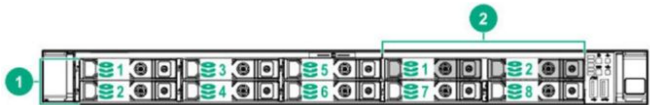
8 SFF + 2 SFF device bay numbering
