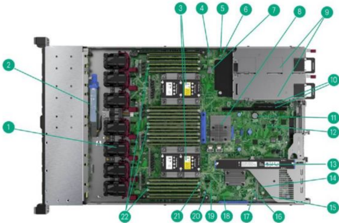
Internal View - Standard for all DL360 Gen10
